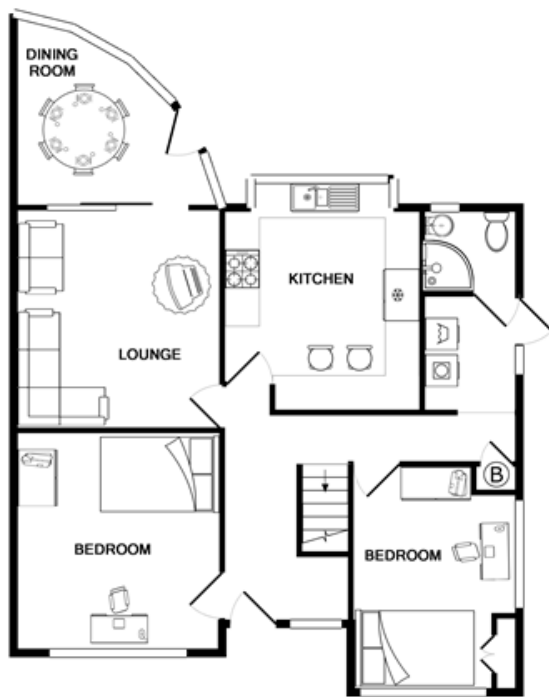
GROUND FLOOR APPROX. FLOOR AREA 80.0 SQ.M. (861 SQ.FT.)
